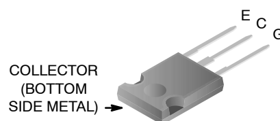
TO-247-3LD SHORT LEAD CASE 340CK JEDEC STYLE
